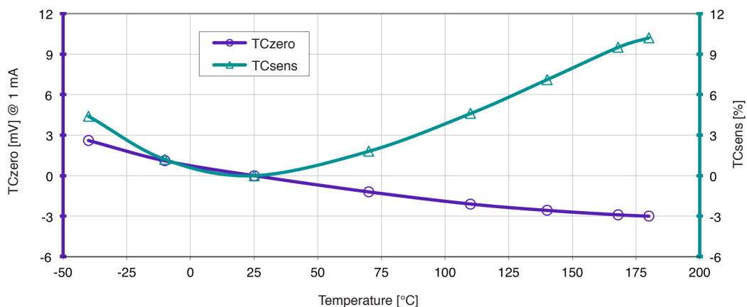
Typical characteristic curve for temperature coefficients (normalised at 25°C)
